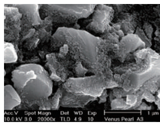
Venus Pearl
